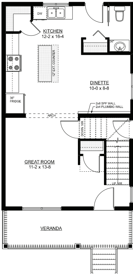
MAIN FLOOR PLAN AREA = 630SQ FT
