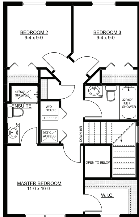
UPPER FLOOR PLAN AREA = 570 SQ FT (EXCLUDES STAIRS/OPEN TO BELOW)
