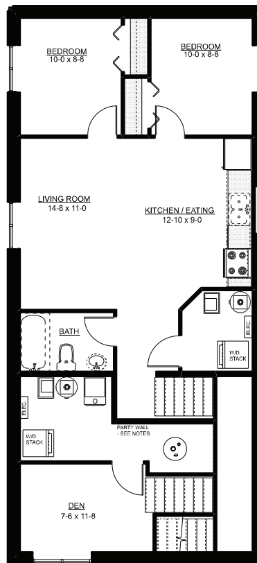
BASEMENT DEVELOPMENT SUITE (SHADED AREA) = 636 SQ FT
