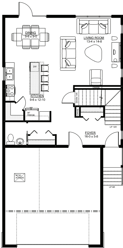
MAIN FLOOR PLAN AREA = 769 SQ FT
