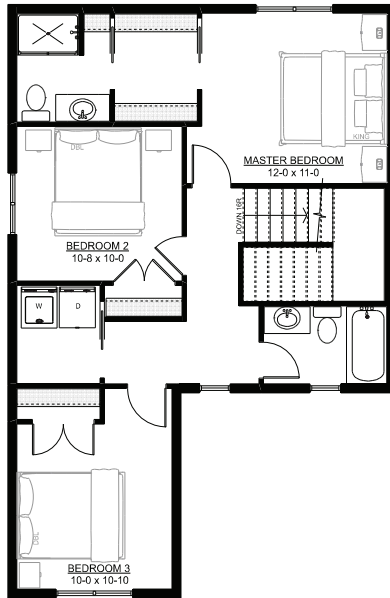
UPPER FLOOR PLAN AREA = 772 SQ FT
