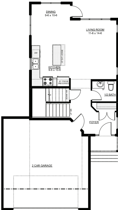
MAIN FLOOR PLAN AREA: 633 SQ FT
